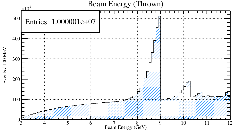
Figure 3.1: A histogram which includes the thrown beam statistics from the generated Monte Carlo example. In the figure one can easily see the coherent peak which maximizes at 9 GeV. Additionally, one can also see other secondary peaks at higher energy.
