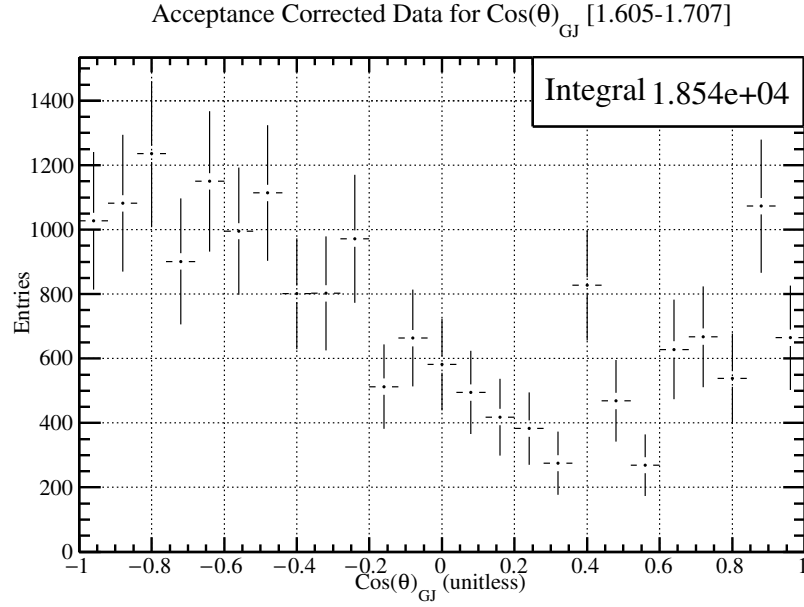
Figure 5.50: The \text{cos}(\theta)_{GJ} distribution for \phi\eta invariant mass between 1.605-1.707 \text{GeV}/c^2 with the acceptance correction factors described in Figure [5.26].
