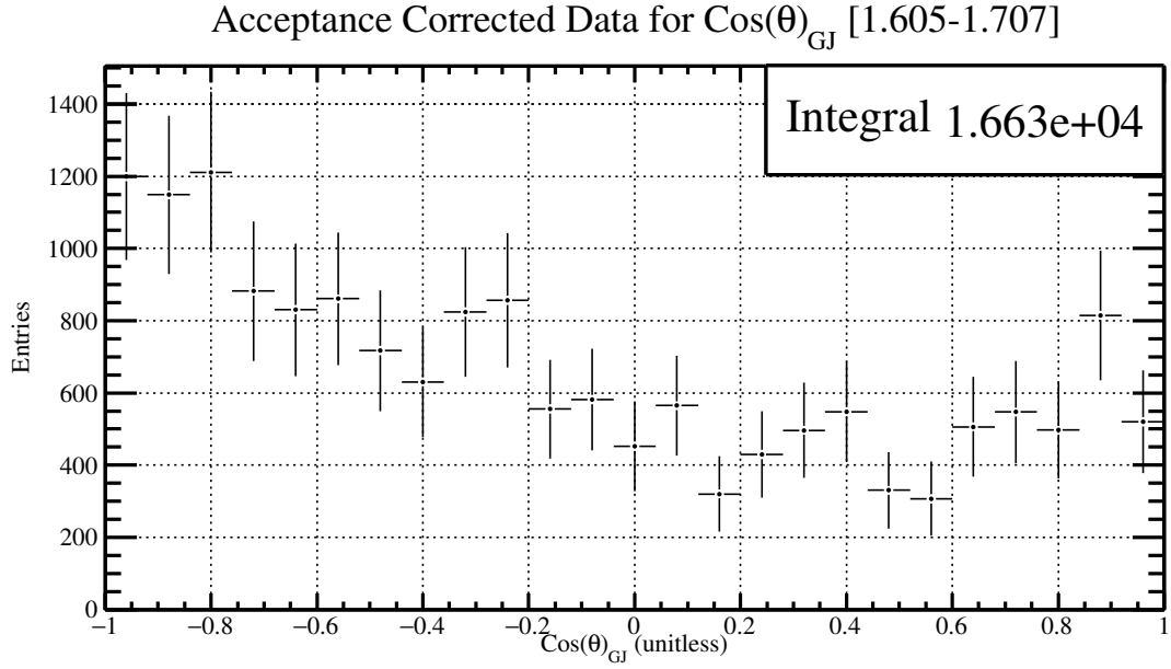
Figure 5.42: The \text{cos}(\theta)_{GJ} distribution for \phi\eta invariant mass between 1.605-1.707 \text{GeV}/c^2 with the acceptance correction factors described in Figure [5.26].
