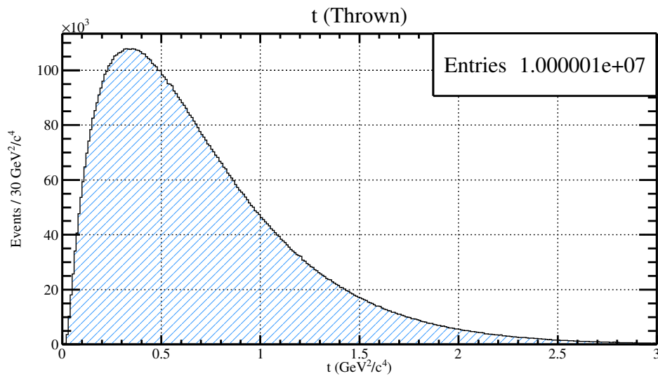
Figure 3.6: A histogram which includes the generated spectrum for the Mandelstam variable, t . The t -slope for the Monte Carlo presented here is 2.5 \frac{GeV^2}{c^4}
