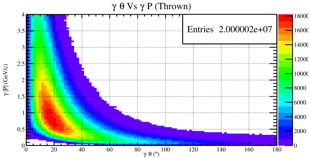
Figure 3.5: A two dimensional histogram which includes the thrown kinematic information of the generated photons. In the histogram, the horizontal axis represents the generated \theta angle in the lab frame, and the vertical axis represents the generated momentum magnitude in the lab frame. The reason that the statistics are doubled in this histogram is due to both final state photon measurements being included in the plot.
