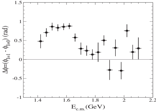
(c) Relative phase difference between the isoscalar and isovector components of the KK^*(892) final state.
