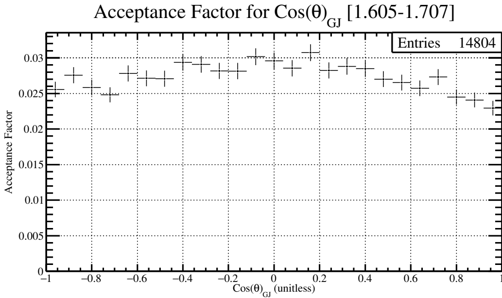
Figure 5.26: The \text{cos}(\theta)_{GJ} acceptance factor for \phi\eta invariant mass range between 1.605-1.707 \text{GeV}/c^2 .
