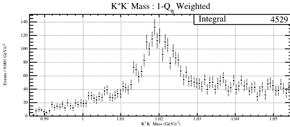
Figure 5.45: The K^+K^- invariant mass spectrum with all events weighted by 1 - Q_\eta .
