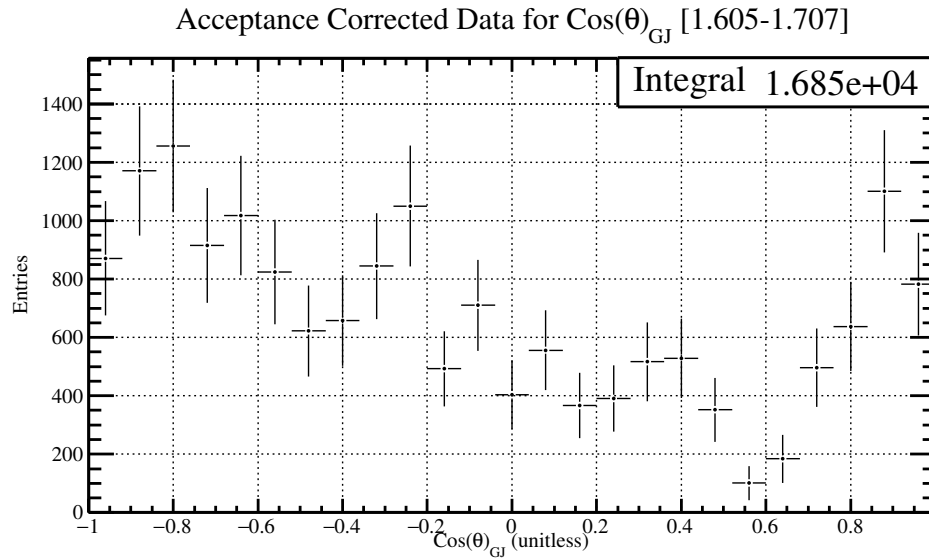
Figure 5.34: The \text{cos}(\theta)_{GJ} distribution for \phi\eta invariant mass between 1.605-1.707 \text{GeV}/c^2 with the acceptance correction factors described in Figure [5.26].
