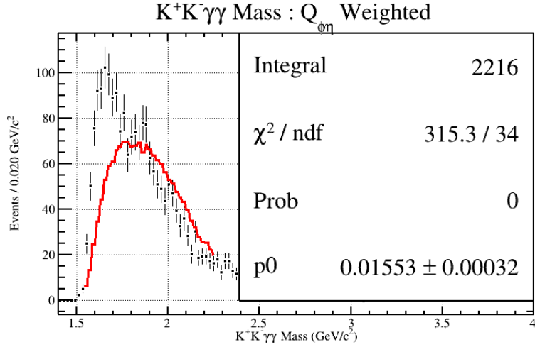
Figure 5.77: Fit of the \phi\eta mass using the Q_{\phi\eta} Weighted distribution in Figure [5.54]. The fit contains no signal distribution, only a scaled accepted Monte Carlo distribution as background. The \chi^2/\text{ndf} , probability, and fit parameters are all given in the stat box.
