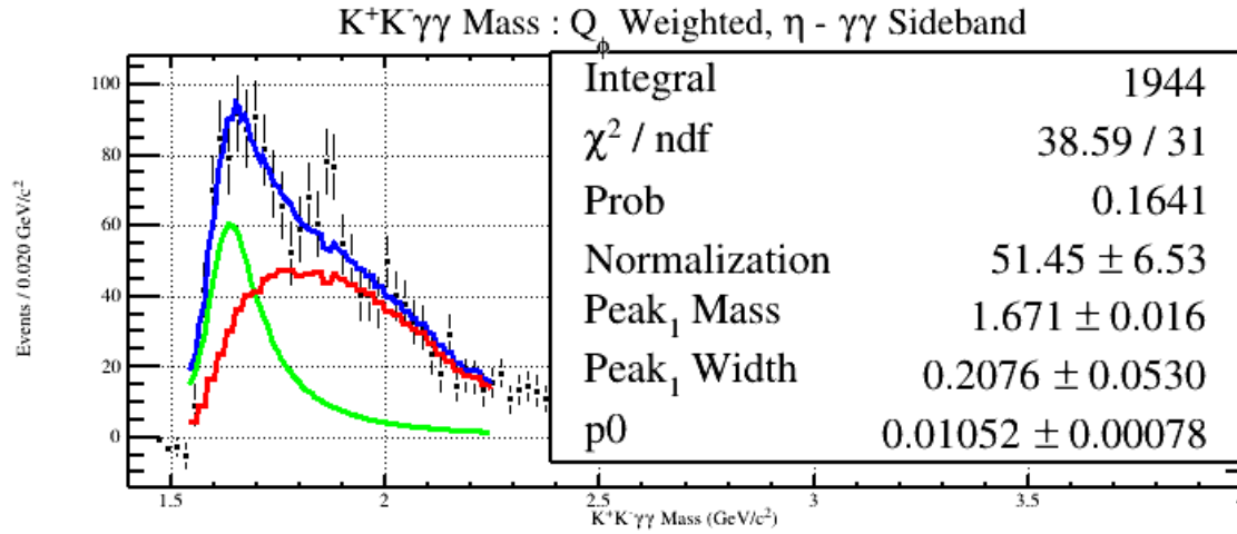
Figure 5.67: Fit of the \phi\eta mass using the Q_\phi Weighted, \eta-\gamma\gamma Sideband distribution in Figure [5.38]. The fit contains one low mass relativistic Breit-Wigner as signal, plus a scaled accepted Monte Carlo distribution as background. The \chi^2/\text{ndf} , probability, and fit parameters are all given in the stat box.
