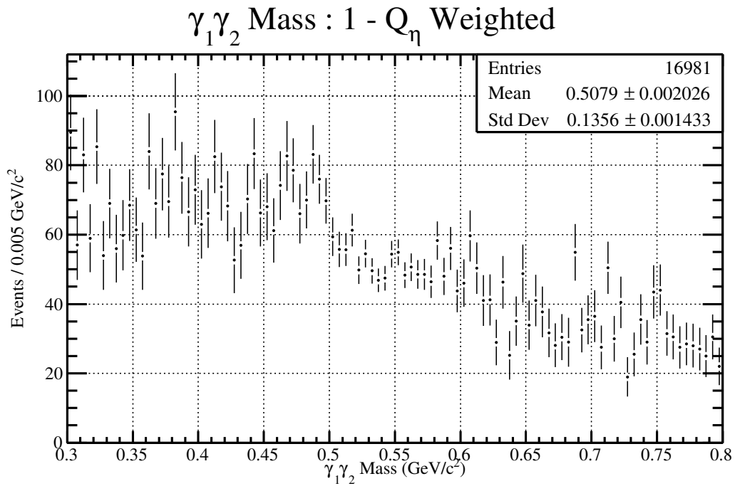
Figure 5.15: The \gamma\gamma invariant mass distribution plotted with the signal weight, Q_\eta and the background weight 1 - Q_\eta .
