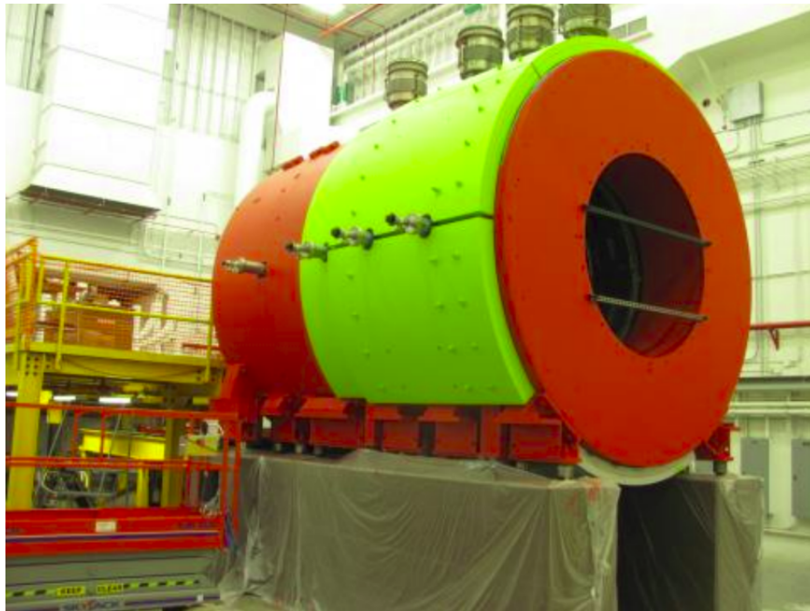
Figure 2.13: A picture taken of the solenoid located inside Hall D. [33]
