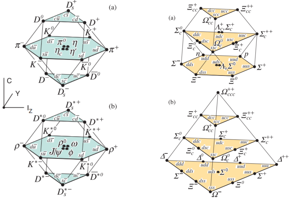
Figure 1.2: (upper-left) J^{PC} = 0^{-+} pseudoscalar meson multiplet. (upper-right) J^{PC} = 1/2^{+} baryon multiplet. (lower-left) J^{PC} = 1^{-+} vector meson multiplet. (lower-right) J^{PC} = 3/2^{+} baryon multiplet
