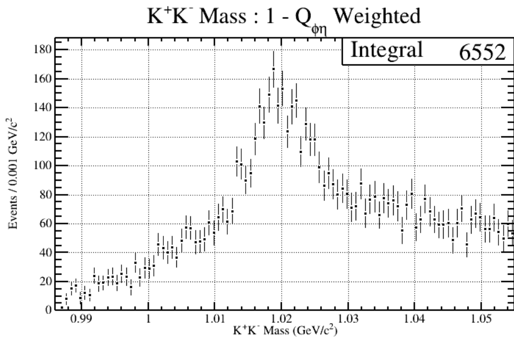
Figure 5.53: The K^+K^- invariant mass spectrum with all signal events weighted by Q_{\phi\eta} , not acceptance corrected.
