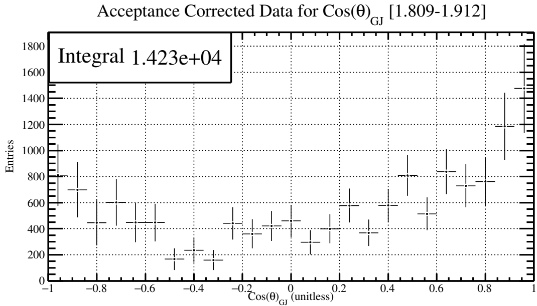
Figure 5.43: The \text{cos}(\theta)_{GJ} distribution for \phi\eta invariant mass between 1.809-1.912 \text{GeV}/c^2 with the acceptance correction factors described in Figure [5.27].
