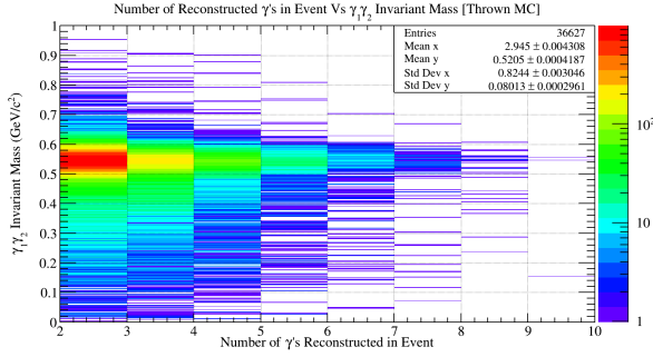
(a) Number of photons reconstructed in an event versus \gamma\gamma Invariant Mass for thrown photons.
