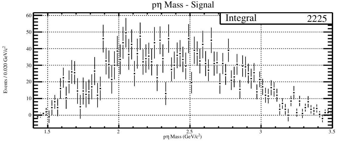
Figure 5.23: The p\eta invariant mass for the Elliptical Subtraction method (Subsec: 5.5.1) after a \theta cut of 18^\circ .
