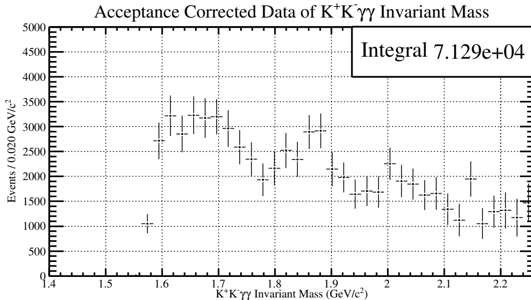
Figure 5.41: The K^+K^-\gamma\gamma invariant mass spectrum with all signal events weighted by Q_\phi , and the \eta is selected by side-band subtraction. The spectrum is acceptance corrected as described by Figure [5.25]. The range of the distribution has been changed due to the large error bars at high \phi\eta invariant mass values.
