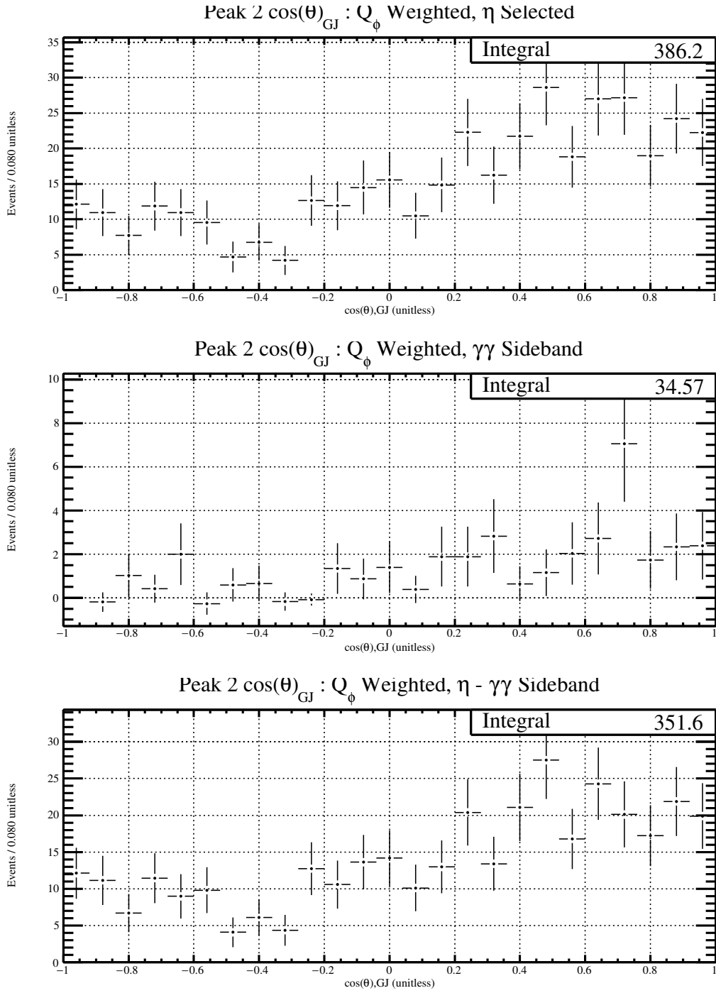
Figure 5.40: The \cos(\theta)_{GJ} distribution for \phi\eta invariant mass between 1.809-1.912 \text{GeV}/c^2 , not acceptance corrected.
