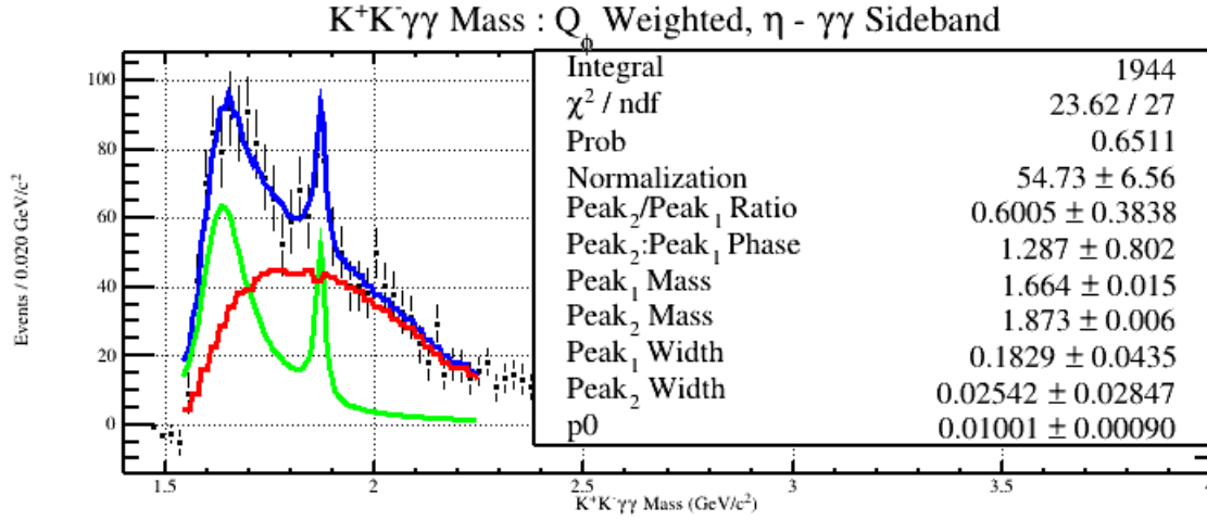
Figure 5.66: Fit of the \phi\eta mass using the Q_\phi Weighted, \eta-\gamma\gamma Sideband distribution in Figure [5.38]. The fit contains two interfering relativistic Breit-Wigners as signal, plus a scaled accepted Monte Carlo distribution as background. The \chi^2/\text{ndf} , probability, and fit parameters are all given in the stat box.
