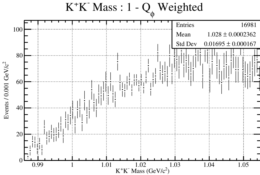
Figure 5.14: The K^+K^- invariant mass distribution plotted with the signal weight, Q_\phi and the background weight 1 - Q_\phi .
