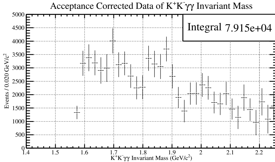
Figure 5.33: The signal \phi\eta invariant mass for elliptical mass selection with the acceptance correction factors described in Figure [5.25]. The range of the distribution has been changed due to the large error bars at high \phi\eta invariant mass values.
