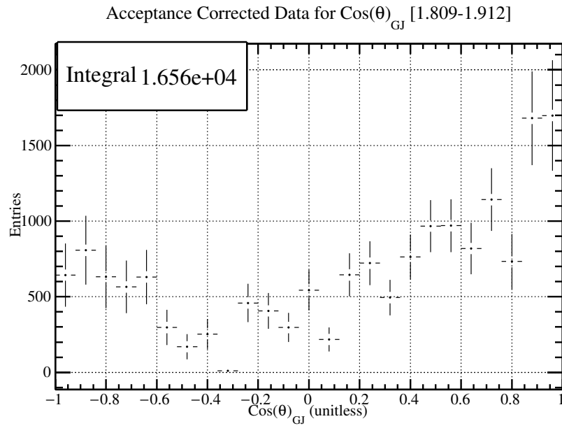
Figure 5.51: The \text{cos}(\theta)_{GJ} distribution for \phi\eta invariant mass between 1.809-1.912 \text{GeV}/c^2 with the acceptance correction factors described in Figure [5.27].
