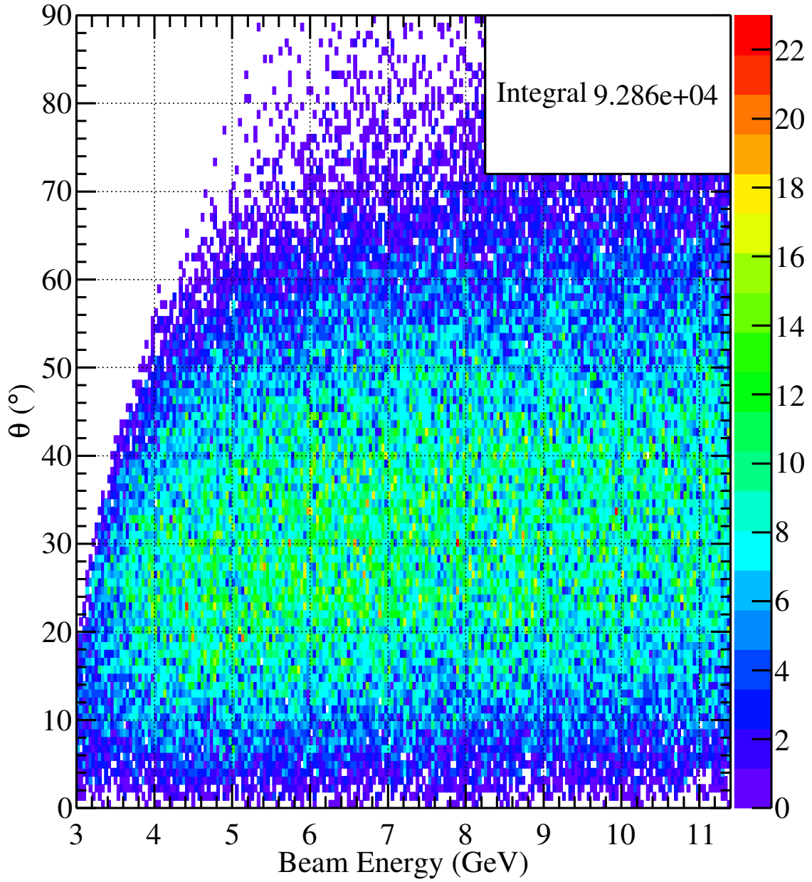
Figure 5.20: The angle of the \eta meson with respect to the beam direction in the lab frame versus the beam energy for \gamma p \rightarrow N^*(1650)\phi; N^*(1650) \rightarrow p\eta Monte Carlo sample.
