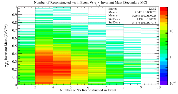
(b) Number of photons reconstructed in an event versus \gamma\gamma Invariant Mass for secondary photons.
